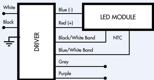
WIRING DIAGRAM
