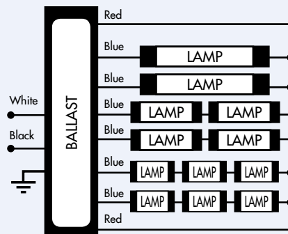
Cap off un-used lead(s) WIRING DIAGRAM 1
