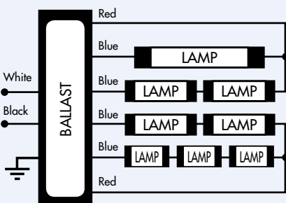
Cap off un-used lead(s) WIRING DIAGRAM 1
