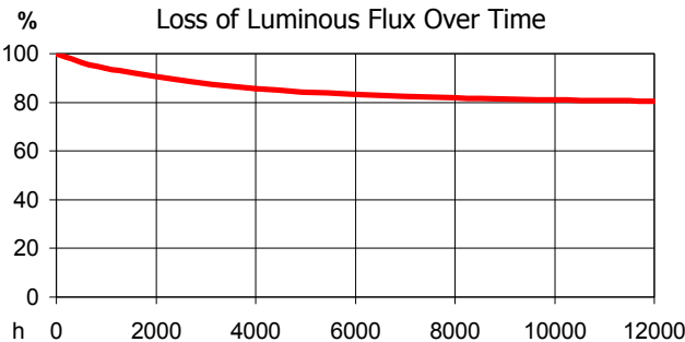
Loss of Luminous Flux Over Time
