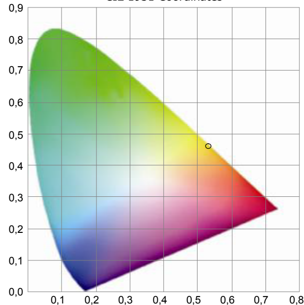
CIE 1931 Coordinates
