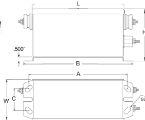
The 9030 P5G-2U has horizontal mounting of primary bushing as shown in diagram above.
